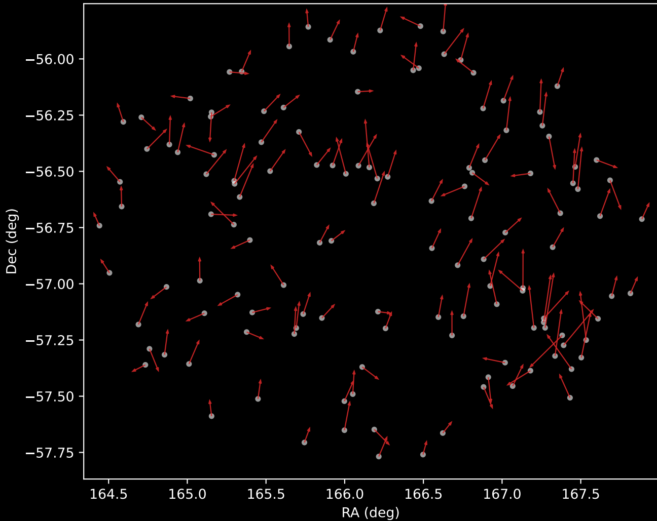
GALAH DR4 Cluster 6 Proper Motion Vectors (n=132)
