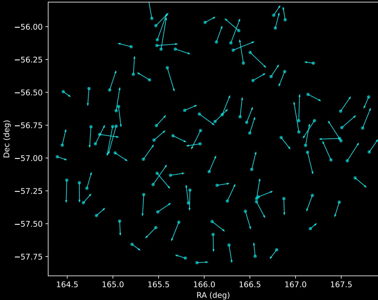
GALAH DR4 Noise Stream Proper Motion Vectors (n=102)
