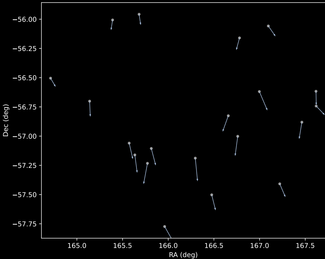
GALAH DR4 Cluster 1 Proper Motion Vectors (n=20)
