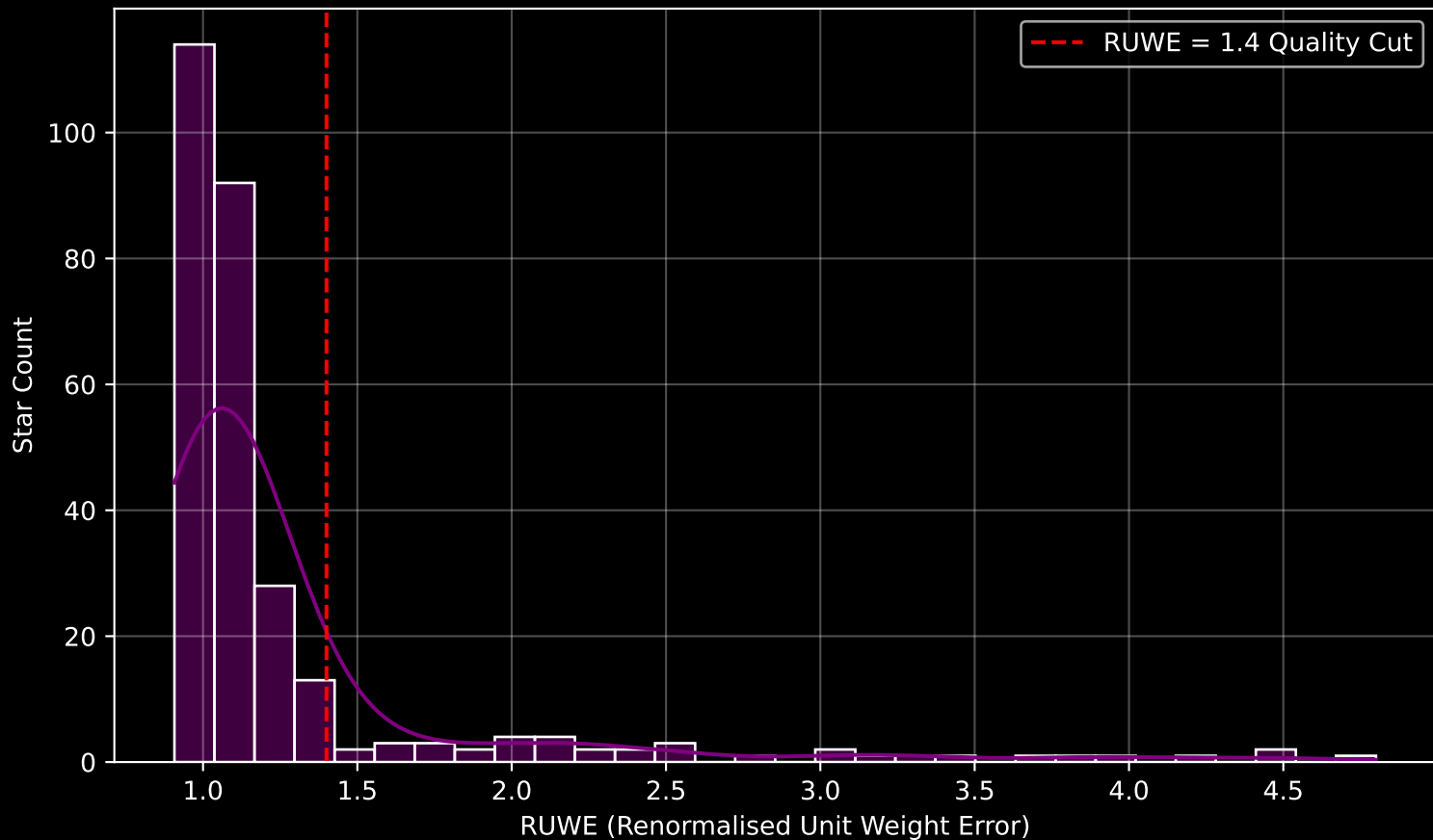
GALAH DR4 Field [150] RUWE Distribution (n= 285)
