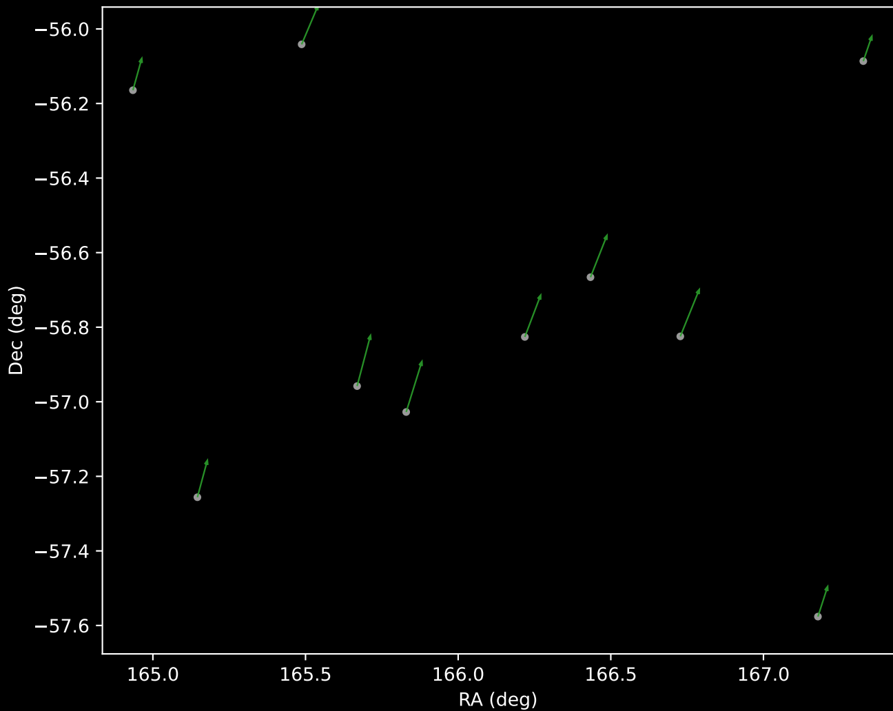
GALAH DR4 Cluster 4 Proper Motion Vectors (n=10)
