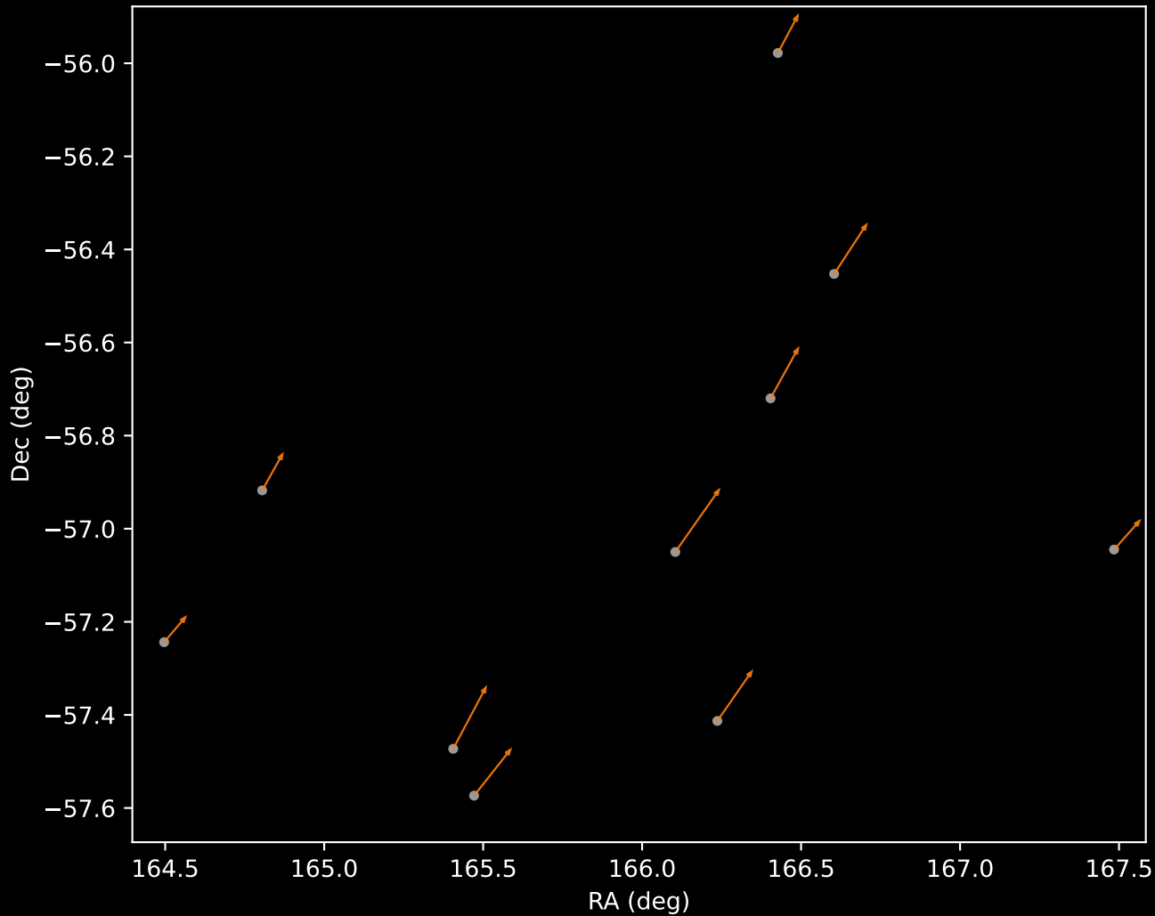
GALAH DR4 Cluster 2 Proper Motion Vectors (n=10)
